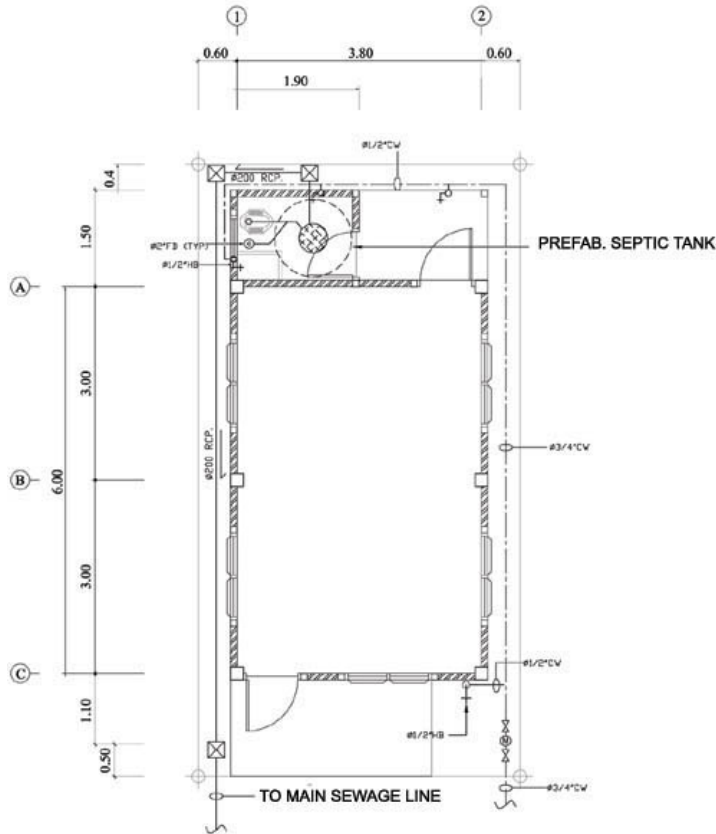
PLUMBING PLAN
