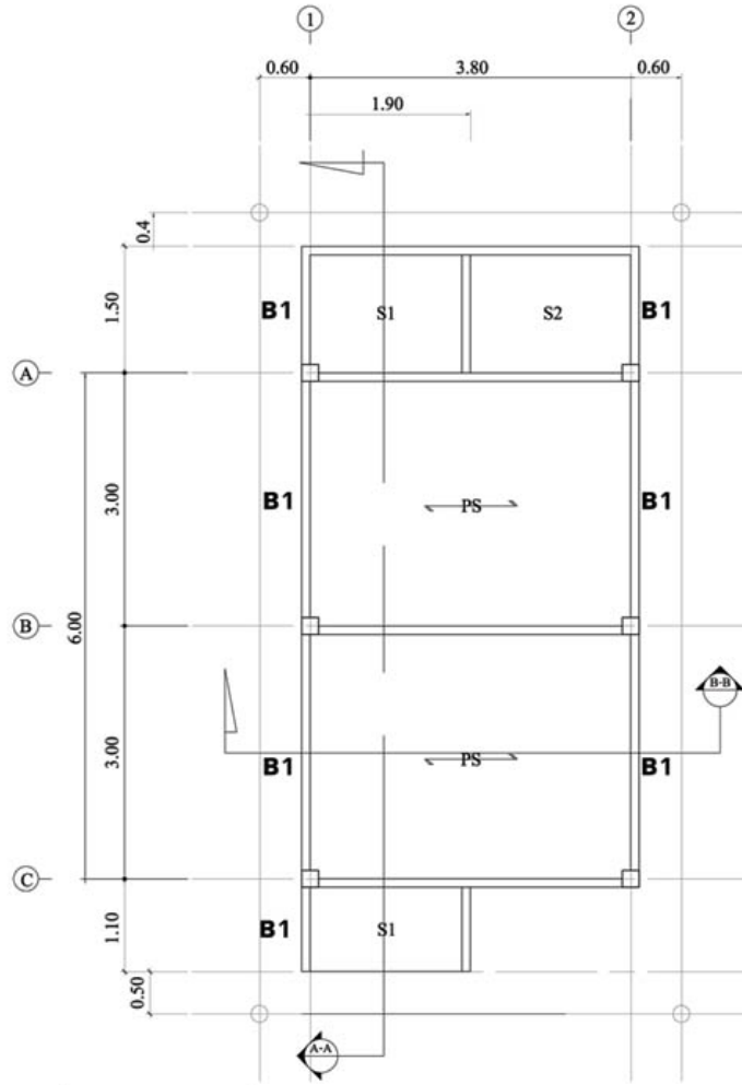
GRADE BEAMS
