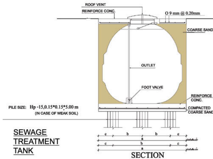
SEPTIC TANK SECTION
