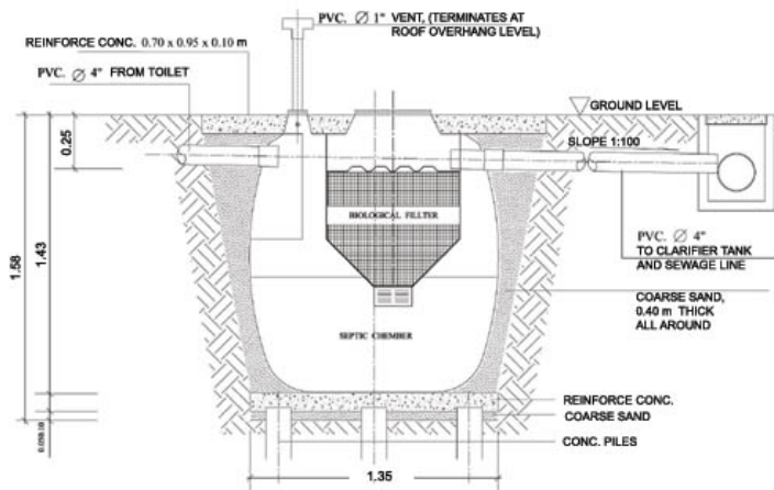
SEPTIC TANK SECTION
